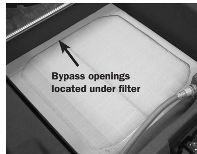
Remove filter, snap bypass cover into position shown, and replace filter.
