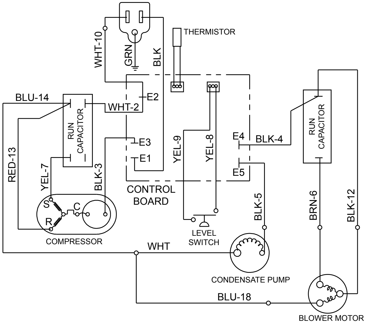
Figure 9: Wiring diagram
